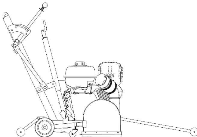
Figure 17-JS SERIES SAWS in cutting operation (Operator wearing personal protective equipment and dust collector are not shown)
