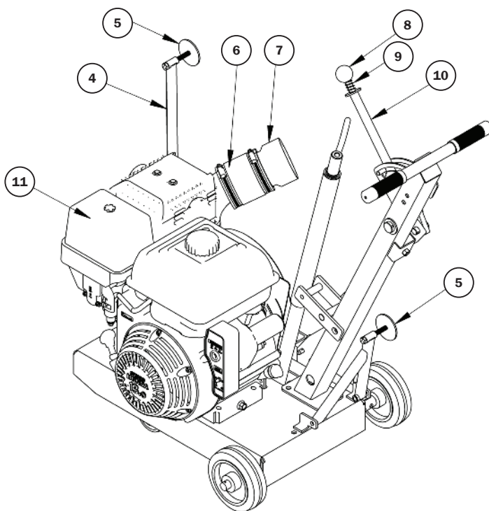
Figure 19 - JS SERIES SAWS top rear left view
