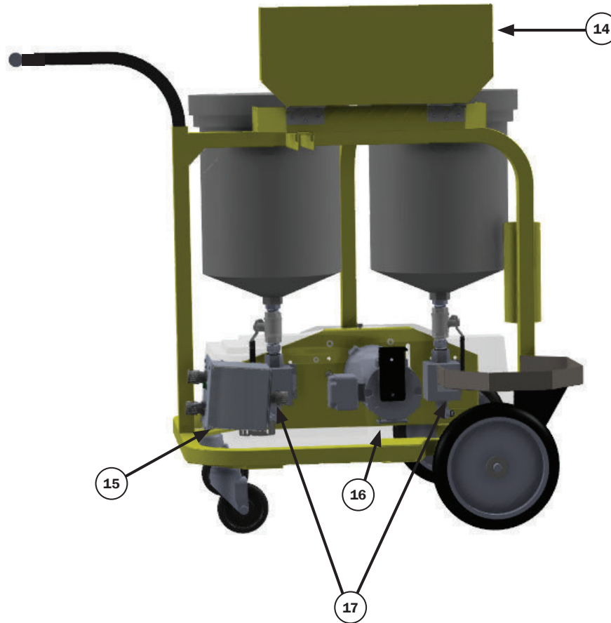
Figure 21 - ONE MAN PUMP with flange detail
